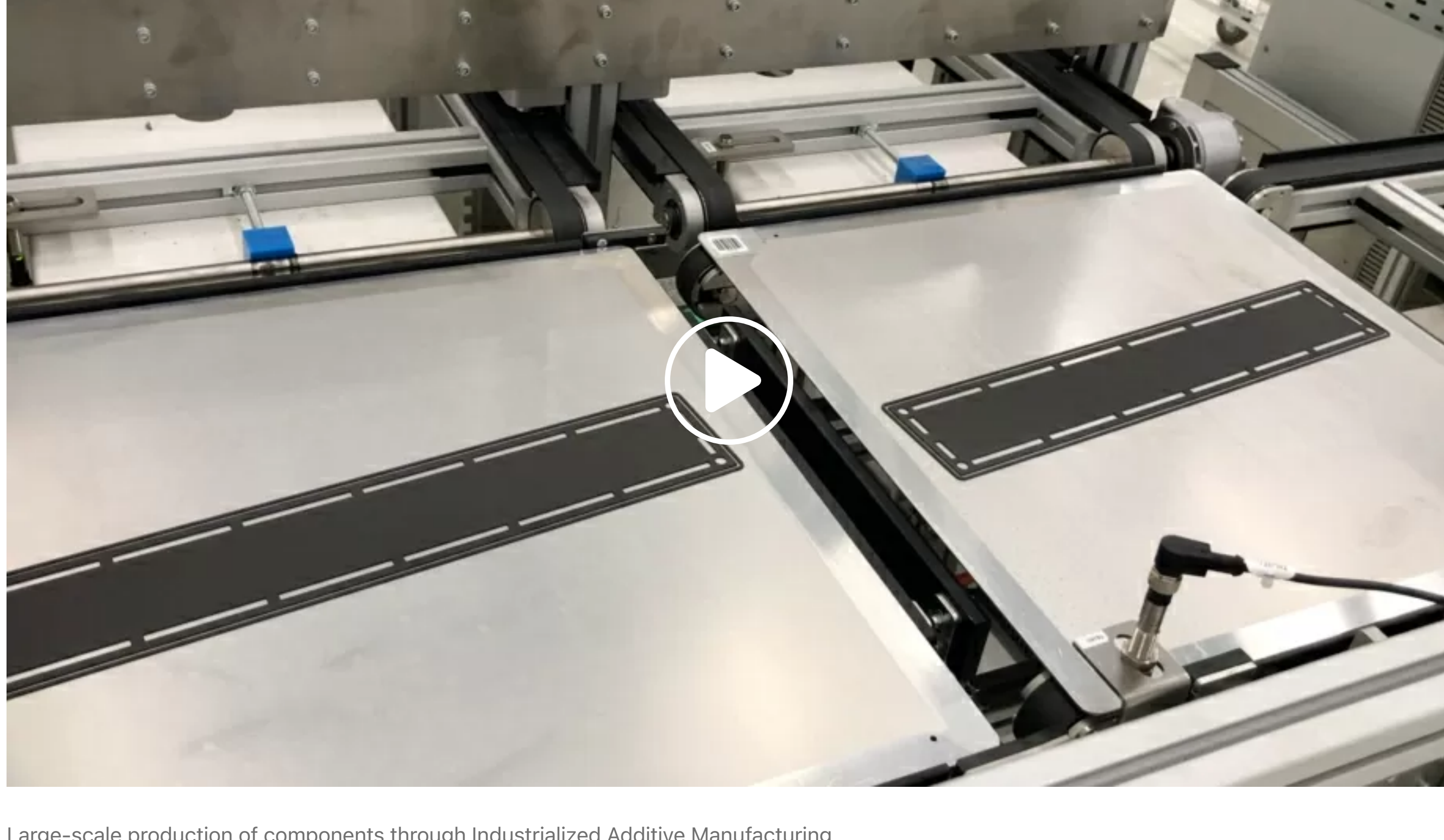
Large-scale production of components through Industrialized Additive Manufacturing
